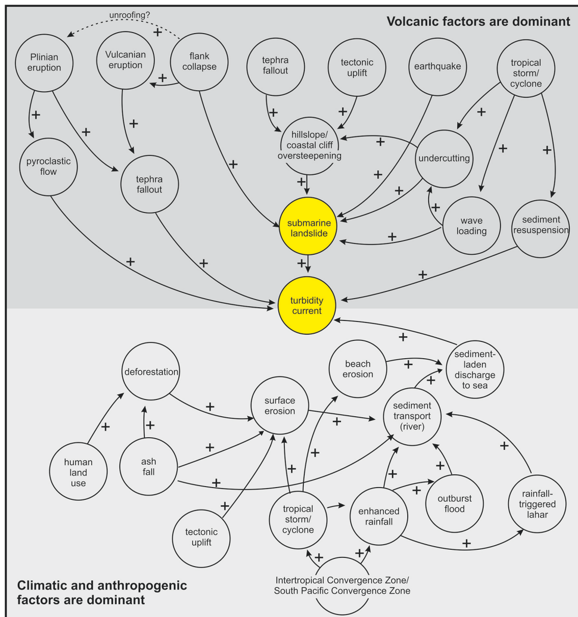
FIGURE 13 | Illustration of the potential complexity of interacting processes at volcanic islands that may precondition and trigger submarine landslides and turbidity currents. Plus signs and arrowed lines indicate how an increase in a variable may make a subsequent process more likely. Figure shows scenarios where volcanic factors may dominate (dark gray) and where climatic or anthropogenic factors may be more important (light gray). An animated version of this figure is available in the online material. Yellow circle refers to ultimately triggered event (landslide or turbidity current).
