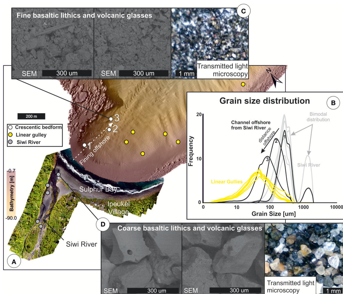
FIGURE 7 | Location of sediment samples presented in this study (A) overlain on drone-acquired photographic survey of Siwi River and multibeam bathymetry offshore. Grain size distributions (B) from Siwi River (gray lines) are similar to those from the proximal part of the sinuous channel with crescentic bedforms (black lines – 1–3), but distinct from samples from linear gullies (yellow lines). Details of SEM and transmitted light microscopy are shown for specific locations (C,D).
