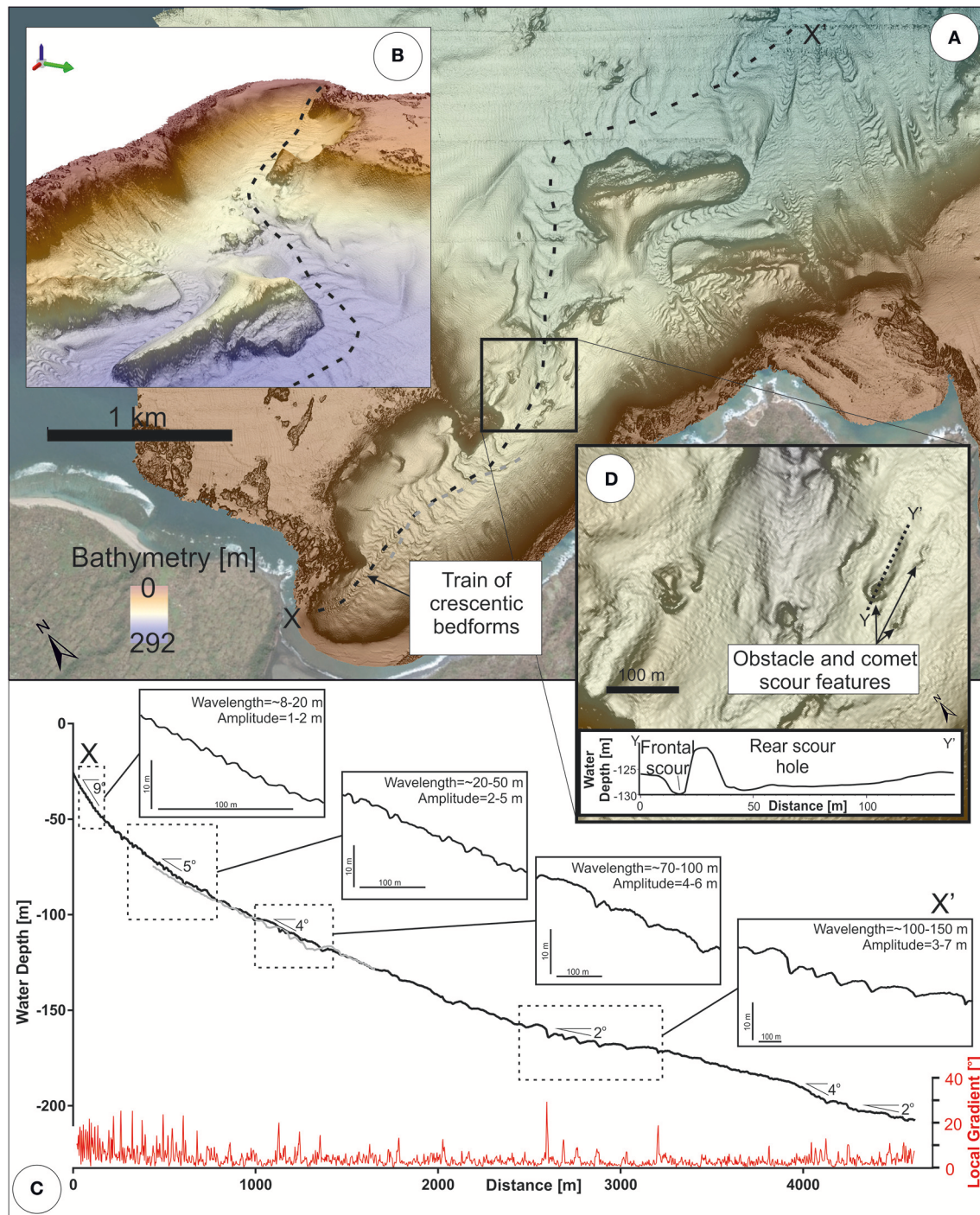
FIGURE 4 | Overview map (A) and 3D rendering (B) annotated with dashed line along the axis of sinuous channel with crescentic bedforms that originates in Sulfur Bay. Along-channel profile (black and gray lines in C) shows how bedforms generally increase in wavelength and amplitude with increasing water depth. Average slope gradients are annotated on the black profile, while local slope gradient that highlights bedforms and knickpoints is shown as a red line in (C). Localized obstacle and scour features are shown in (D).
